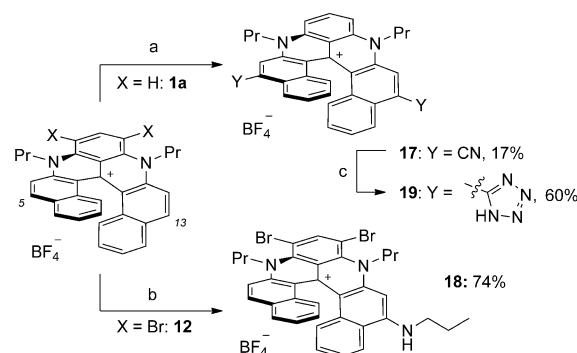
Scheme 4. a) NaCN (3 equiv), DMF, 60 h, 25°C; b) n -PrNH 2 , 16 h, 25°C; c) TMSN 3 (3 equiv), Bu 2 SnO (20%), PhCl, 16 h, 60°C. DMF = N,N -dimethylformamide, TMS = trimethylsilyl.
