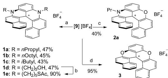
Scheme 2. Reagents and reaction conditions: a) Anhydrous RNH 2 (25 equiv), NMP, MW 170°C, 10 min; b) PPh 3 , DIAD, CH 3 COSH, THF, 25°C; c) n -PrNH 2 , 49°C, 30 min, then heated neat at 200°C, 5 min; d) Pyr-HCl, 224°C, 2 min then ion exchange metathesis with HBF 4 . DIAD = diisopropyl azodicarboxylate, MW = microwave, NMP = N -methyl-2-pyrrolidone, THF = tetrahydrofuran.
