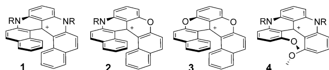
Figure 1. The cationic diaza 1 , azaxo 2 , and dioxo 3 [6]helicenes, and the [4]helicene quinacridinium derivatives of type 4 . Only the P enantiomers are shown. R = alkyl chains.
