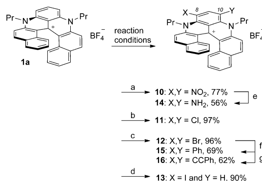
Scheme 3. Reagents and reaction conditions: a) HNO 3 , 15 min, 25°C; b) NCS (3 equiv), CHCl 3 , AcOH, 15 h, 25°C; c) NBS (3 equiv), CHCl 3 , AcOH, 15 h, 25°C; d) NIS (3 equiv), CHCl 3 , AcOH, 15 h, 25°C; e) H 2 , PtO 2 (10 wt %), EtOH, 1 h, 25°C; f) [Pd(PPh 3 ) 4 ] (10%), PhB(OH) 2 (5 equiv), K 2 CO 3 (5 equiv), 1,4-dioxane, 15 h, 80°C; g) [Pd(PPh 3 ) 4 ] (20%), CuI (30%), PhC≡CH (10 equiv), Et 3 N, 3 h, 90°C. NBS = N -bromosuccinimide, NCS = N -chlorosuccinimide, NIS = N -iodosuccinimide.
